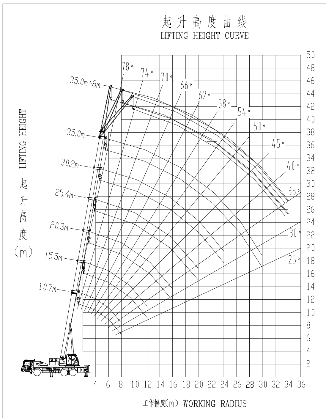
Figure 1-12 Lifting height chart
